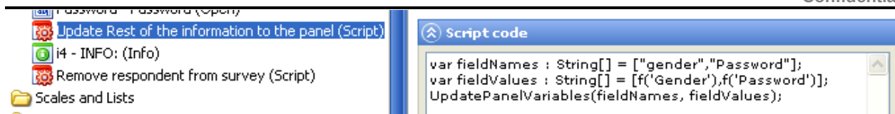
Figure 276 Example of the database registration script
