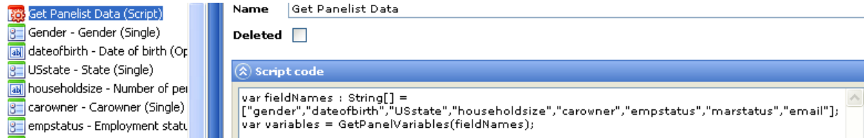
Figure 279 Example of script to fetch the data from the database
