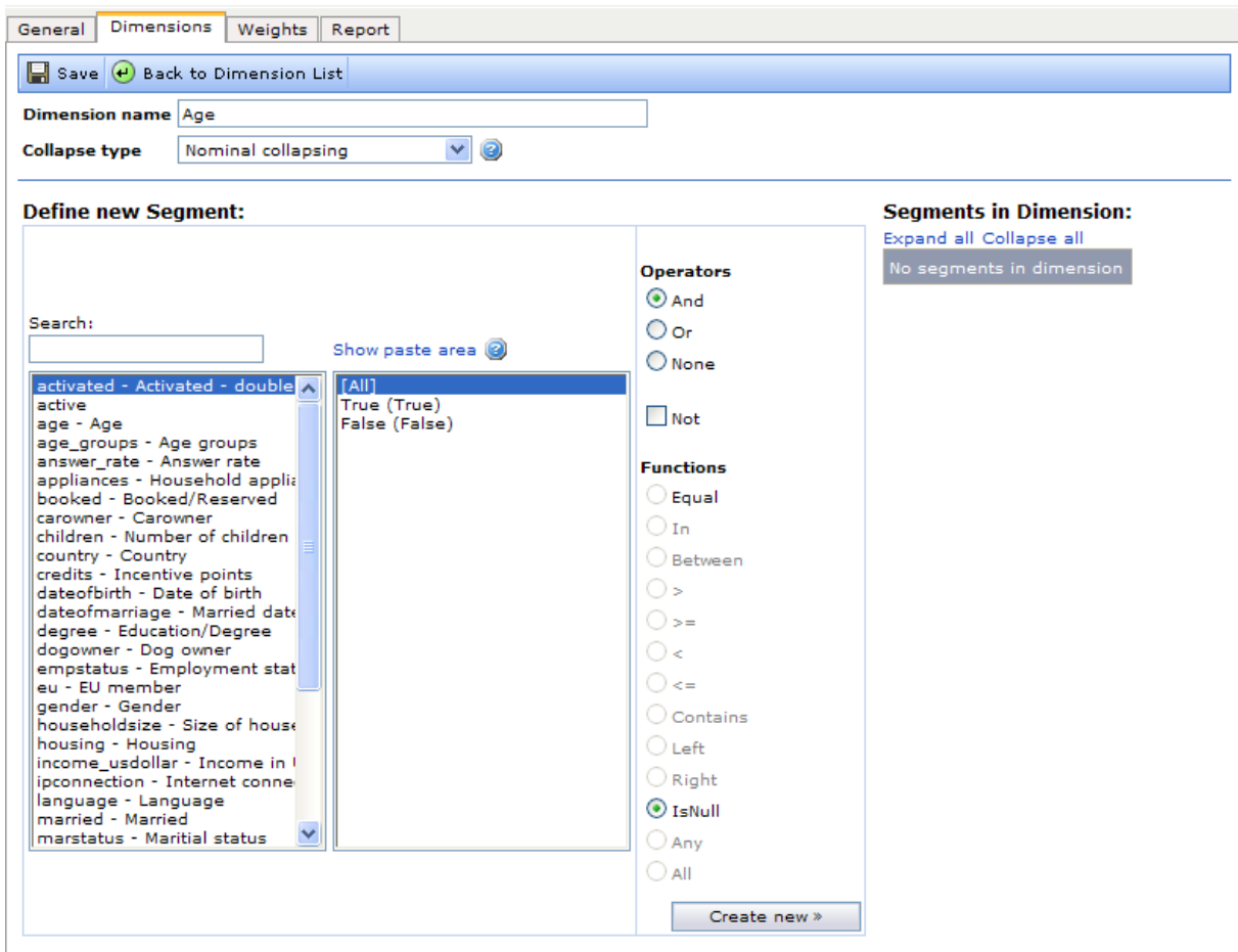
Figure 226 Example of the Edit Dimension window
