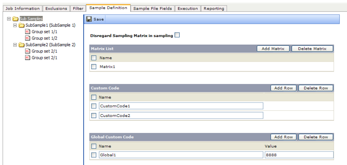
Figure 170 Example of the editing page for the Sub Samples folder
