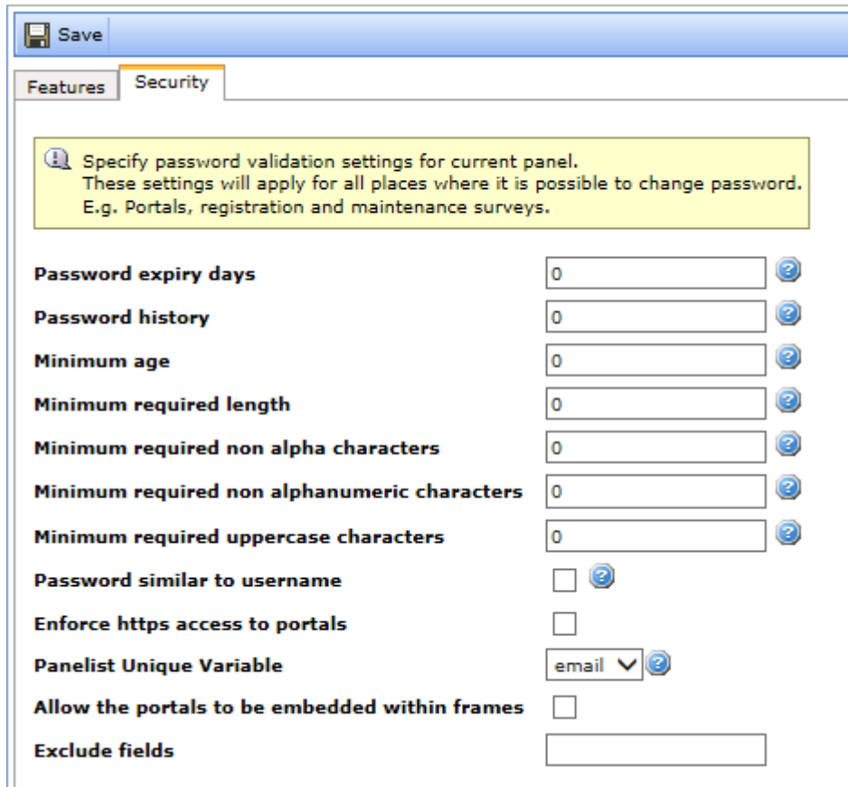
Figure 147 The Panel Settings Security tab
