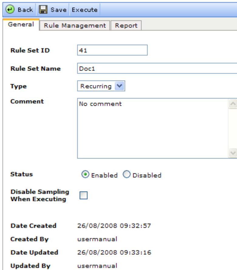
Figure 106 Example of the Rule Set Details page > General tab
