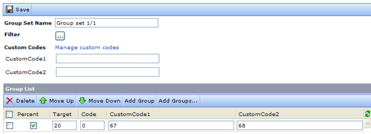
Figure 172 Example of the Group Set editing page
