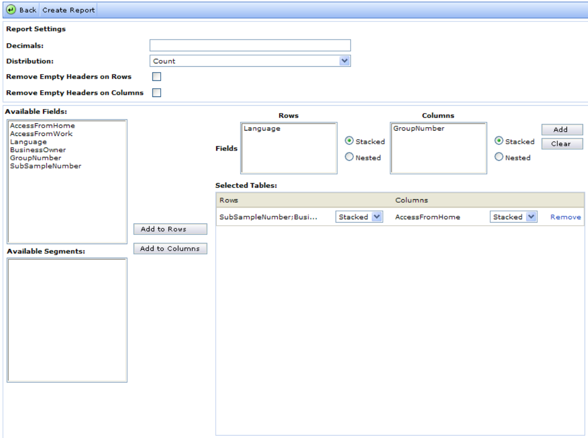
Figure 208 Example of a Crosstab Report under construction
