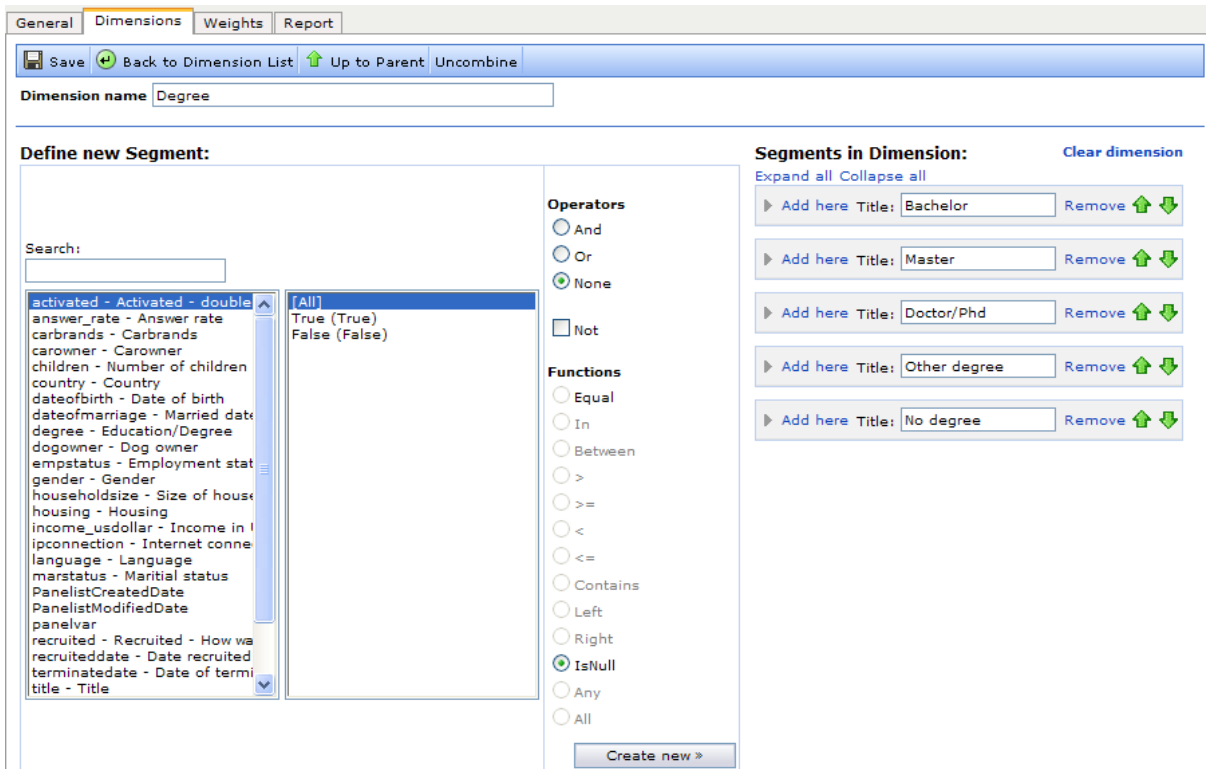
Figure 215 Example of the Edit Dimension page for a dimension
