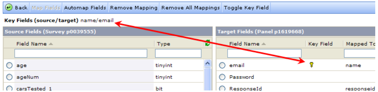
Figure 105 Toggling the key fields
