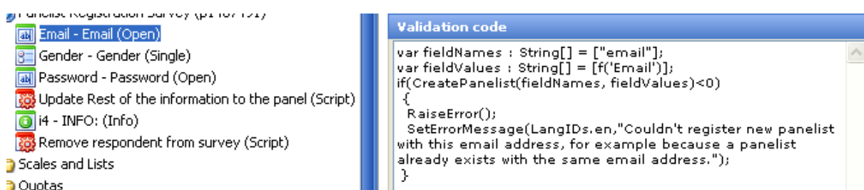
Figure 281 Example of script to check whether the email address already exists
