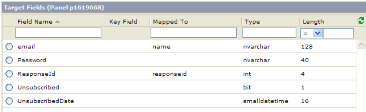
Figure 104 Two fields from the source are mapped to fields in the target
