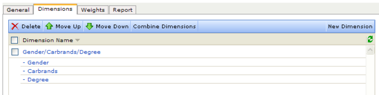
Figure 214 Example of the Dimensions tab list
