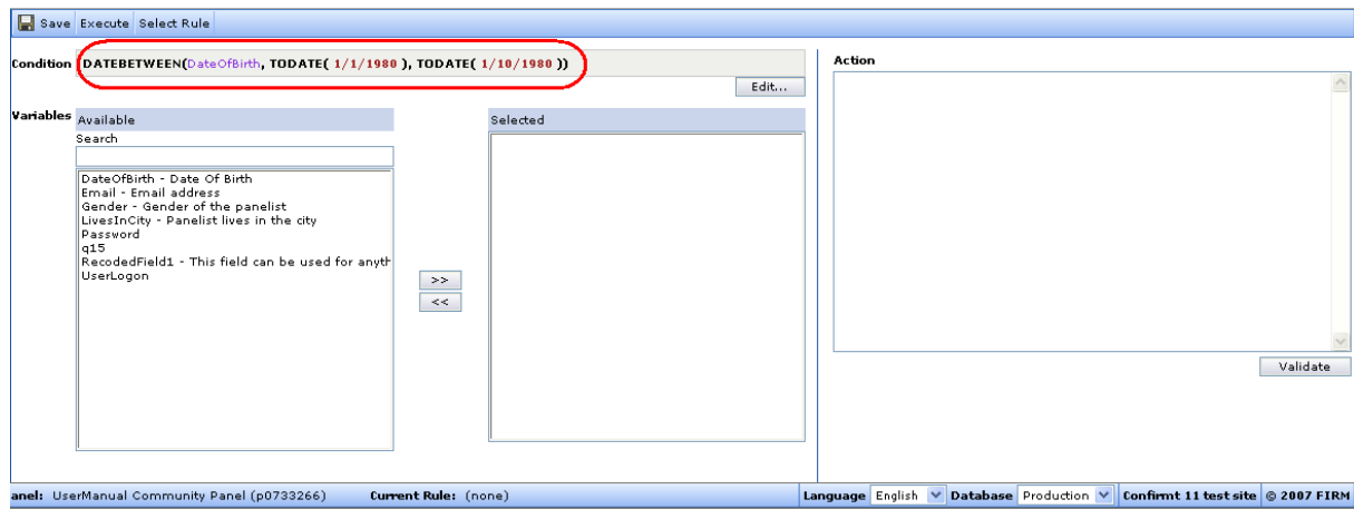
Figure 132 The Panelist Editor with the condition
