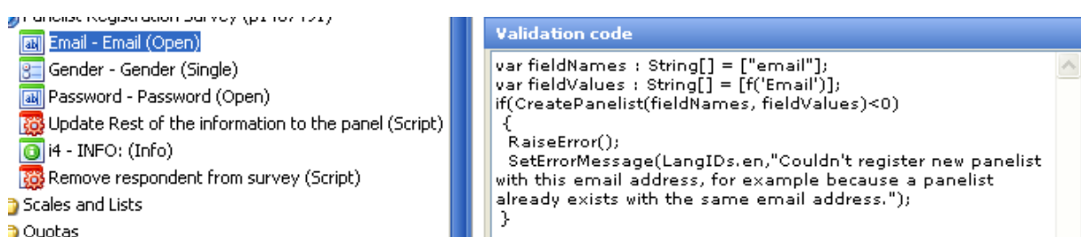
Figure 277 Example of script to check whether the email address already exists
