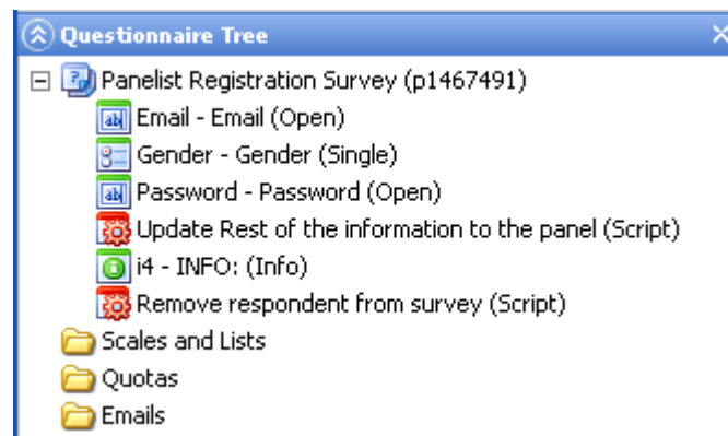
Figure 276 Example of a simple Panelist Registration survey
