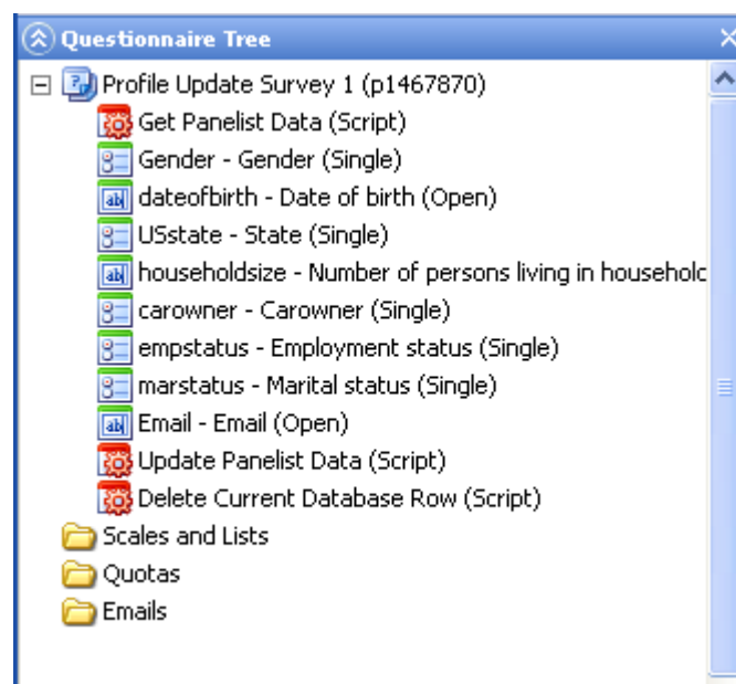
Figure 280 Example of a simple Panelist Update survey
